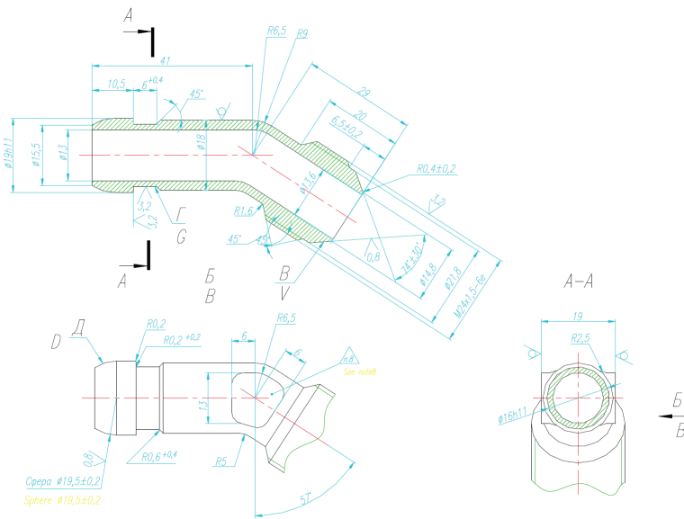
Fig. A – fabrication diagram of the hydraulic joint
